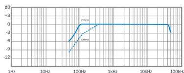
Frequency Response of SR40 (typical)
