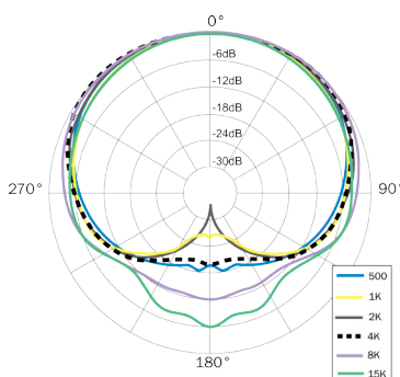
Polar Response of SR40 (typical)
